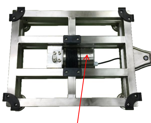
Protection of load cell from water entry
